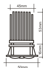
TRIO PF MR 16 Flat Precision
