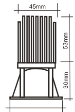
TRIO P MR 16 Diffused
