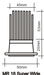
MR 16 Super Wide
