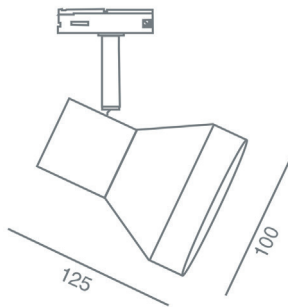
LED PAR30
